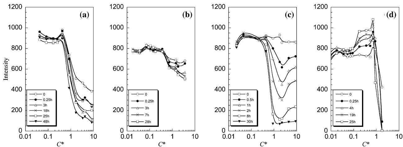
Fig. 1 Scattering intensity of DPPC vesicles in each surfactant solution as a function of the reduced surfactant concentration at various times after mixing. a SDS, b SDSfo, c SDSar, d SDG
