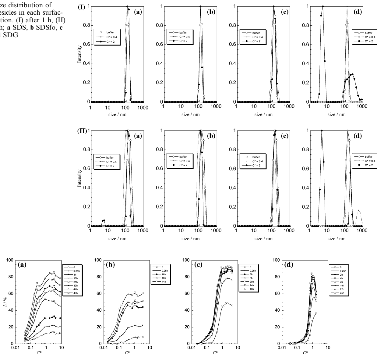
Fig. 3 Leakage ratio of CF from DPPC vesicles versus reduced surfactant concentration curves in each surfactant solution at various times after mixing. a SDS, b SDSfo, c SDSar, d SDG
