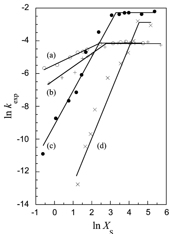
Fig. 5 \ln k_{\text{exp}} versus \ln X_S plots for each surfactant solution. a SDS, b SDSfo, c SDSar, d SDG
